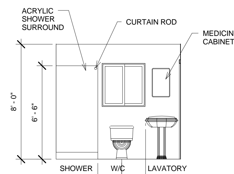
⑤ BATHROOM #3 - A 1/4" = 1'-0"
