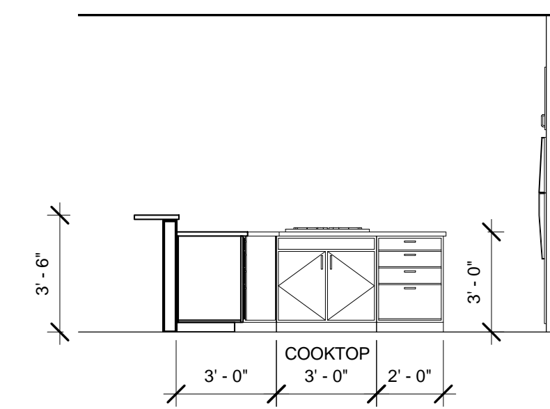
4 KITCHEN - D 1/4" = 1'-0"
