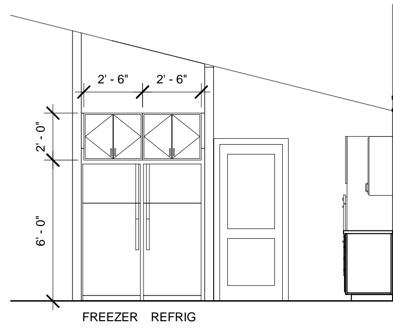
1 KITCHEN - A 1/4" = 1'-0"
