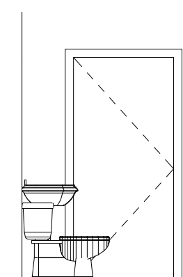
⑥ BATHROOM #3 - B 1/4" = 1'-0"
